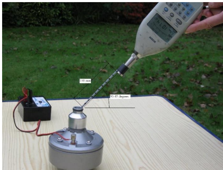
Fig 1: Reference measurement at a distance of 10 cm from the adapter opening.
