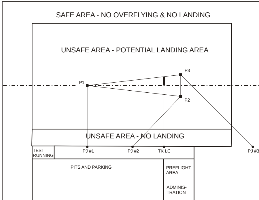
F3E Competition Site Layout - Left
