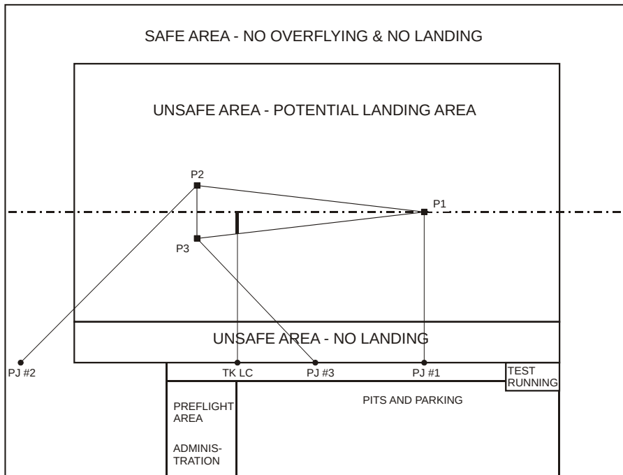
F3E Competition Site Layout - Right
