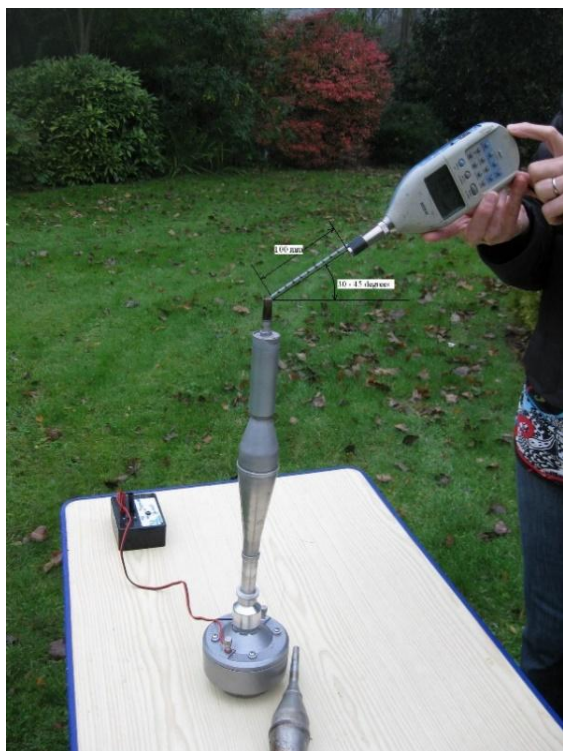
Fig. 2: Measurement of the exhaust system.
